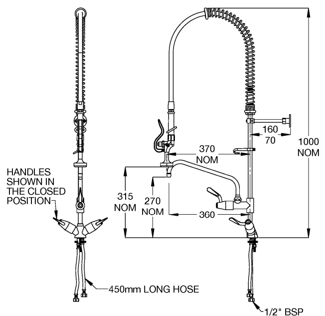
TF100HJP - Assembly
