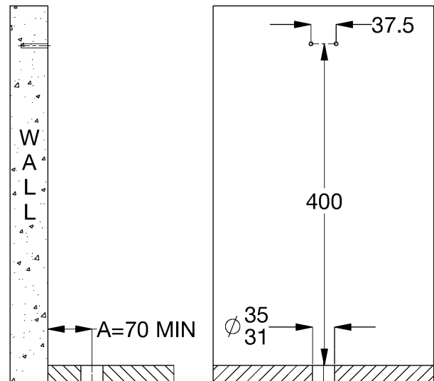
MOUNTING DETAILS
